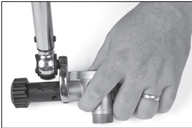
Unscrew the packing nut from the regulator body.
