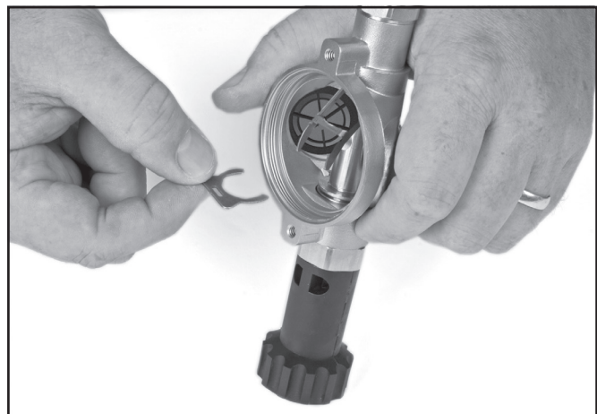
Remove the lock clip from the interior of the regulator.
