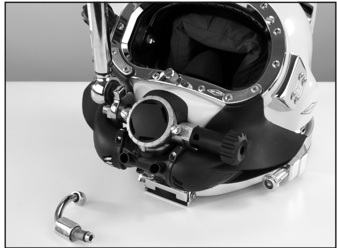
Remove the bent tube and the bent tube adapter on the regulator inlet.
